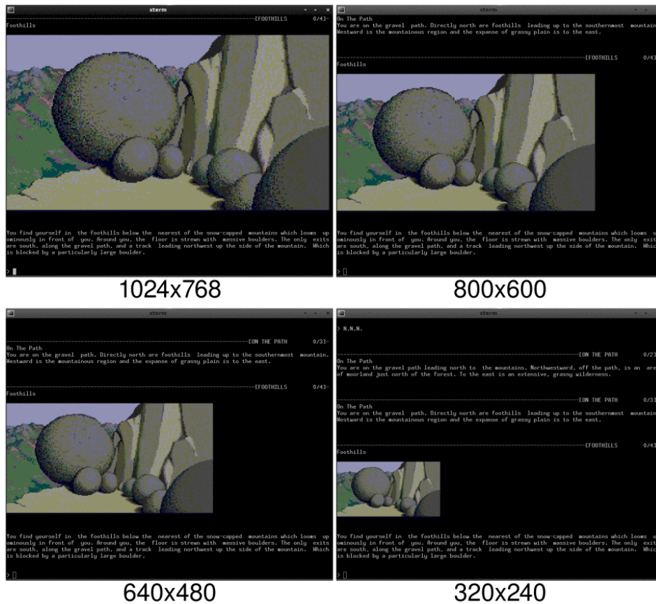
Figure 3.5: Different options for the -sres commandline parameter whilst running the -vmode sixel mode. The original images are being scaled up, their aspect ratio is being preserved. It is up to the user to decide which one should be preferred.
